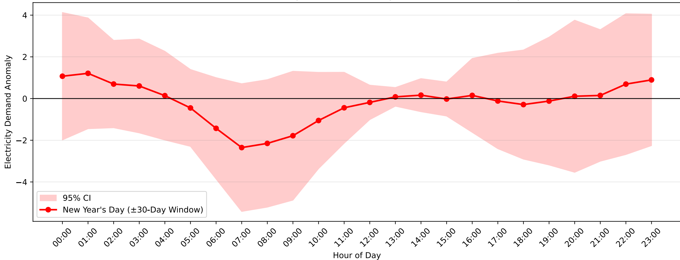
Blakehurst Demand Anomaly: New Year's Day (2010-2011, \pm 30 -Day Window)
