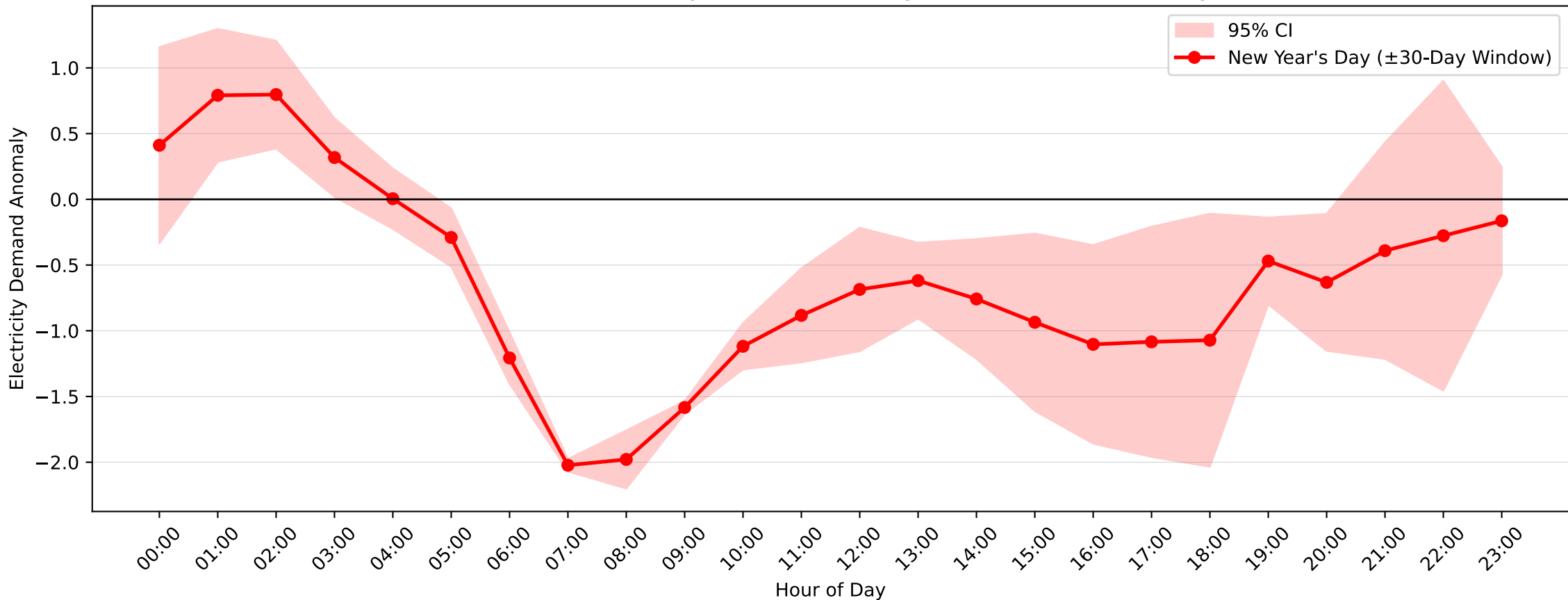
Blakehurst Demand Anomaly: New Year's Day (2013-2014, \pm 30 -Day Window)
