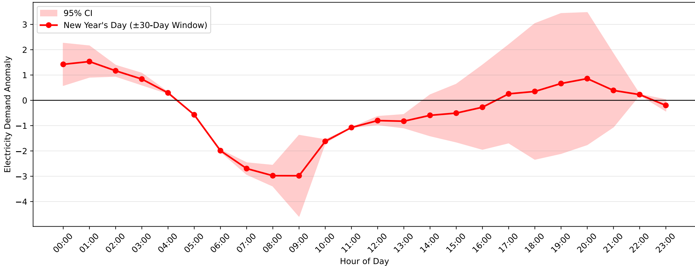
Blakehurst Demand Anomaly: New Year's Day (2008–2009, \pm 30 -Day Window)
