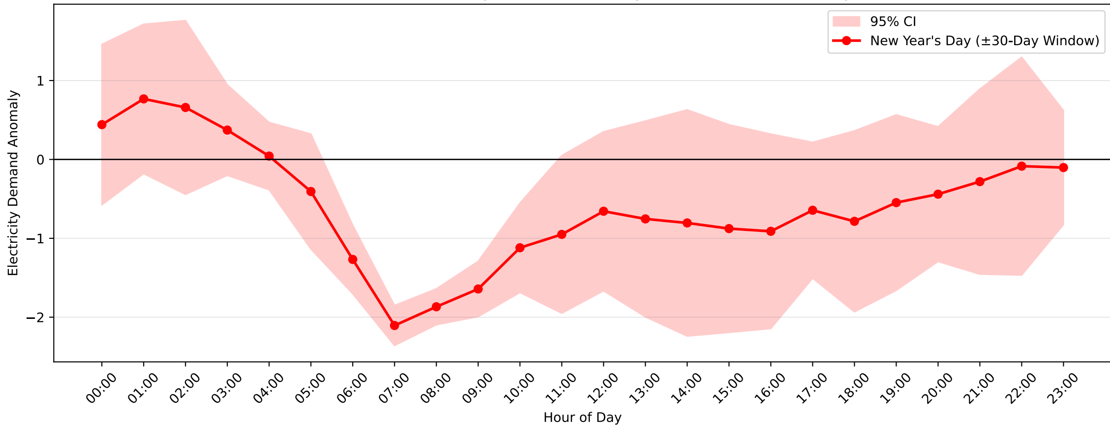
Blakehurst Demand Anomaly: New Year's Day (2012–2013, \pm 30 -Day Window)
